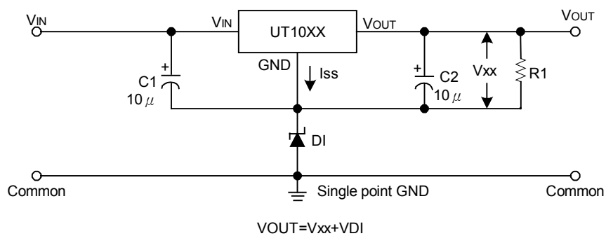
Circuit for increasing output voltage
