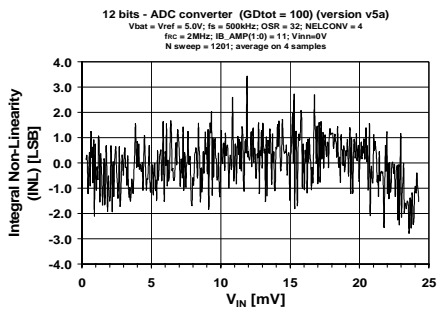
Figure 8.8: GAIN=100, 12 bit ADC setting
