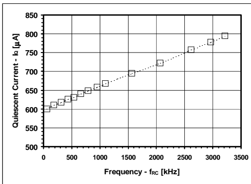
Figure 8.21: Absolute and (b) relative change in quiescent current consumption vs. clock speed
