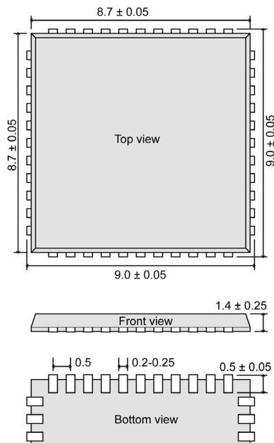
Figure 9.2: PLL-44L package,
