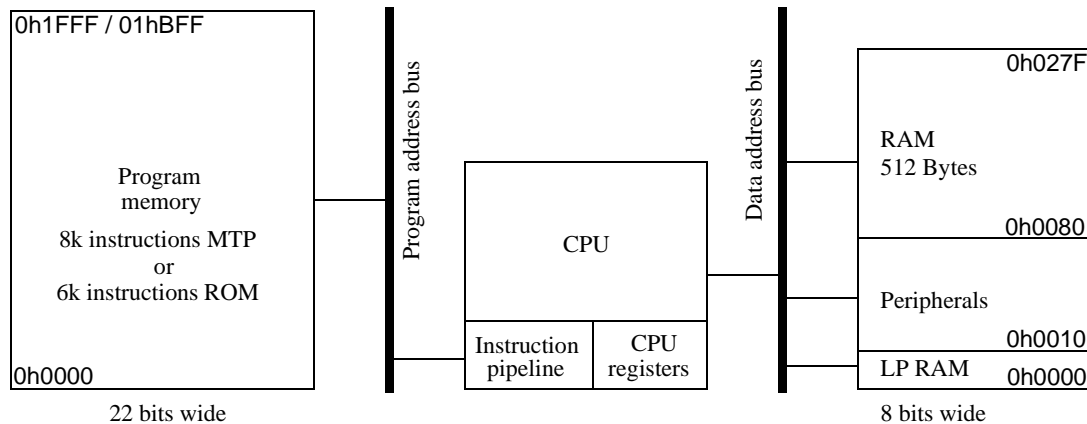
Figure 5.1: Memory organization
