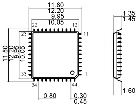
Figure 9.1: LQFP44 package, size in mm.
