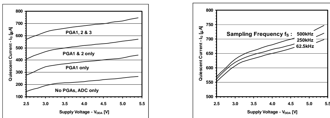
Figure 8.19: Quiescent current versus supply voltage for different gains and clock speed (not using the PGA and ADC low power modes)
