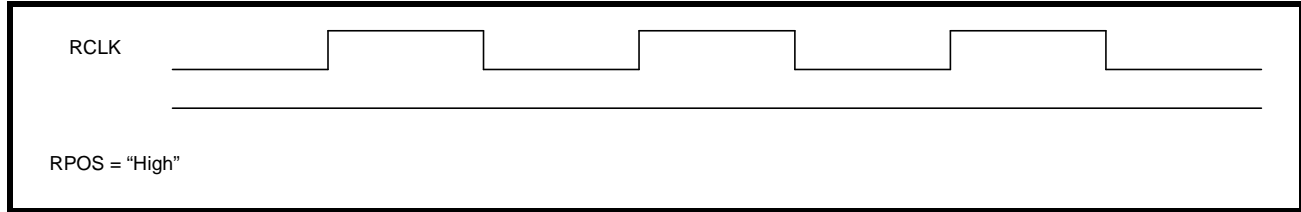
FIGURE 10. SYSTEM SIDE SAIS RECEIVE OUTPUT
