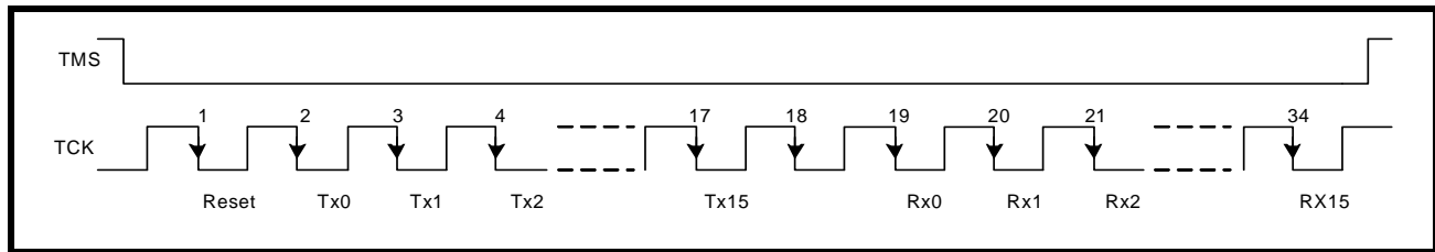
FIGURE 34. TIMING DIAGRAM FOR ATP TESTING
