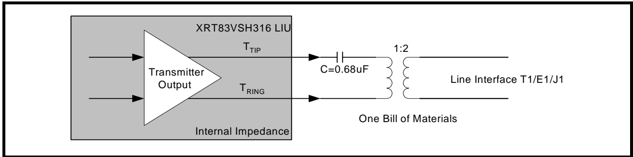
FIGURE 22. TYPICAL CONNECTION DIAGRAM USING INTERNAL TERMININATION
