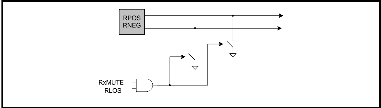
FIGURE 15. SIMPLIFIED BLOCK DIAGRAM OF THE RxMUTE FUNCTION
