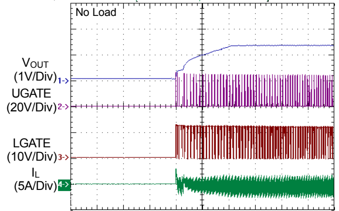
Time (1ms/Div)
