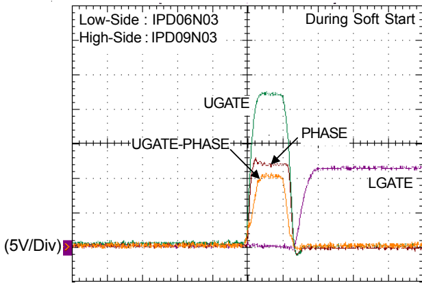
Time (100ns/Div)
