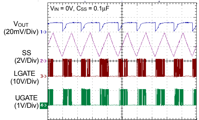
Time (50ms/Div)
