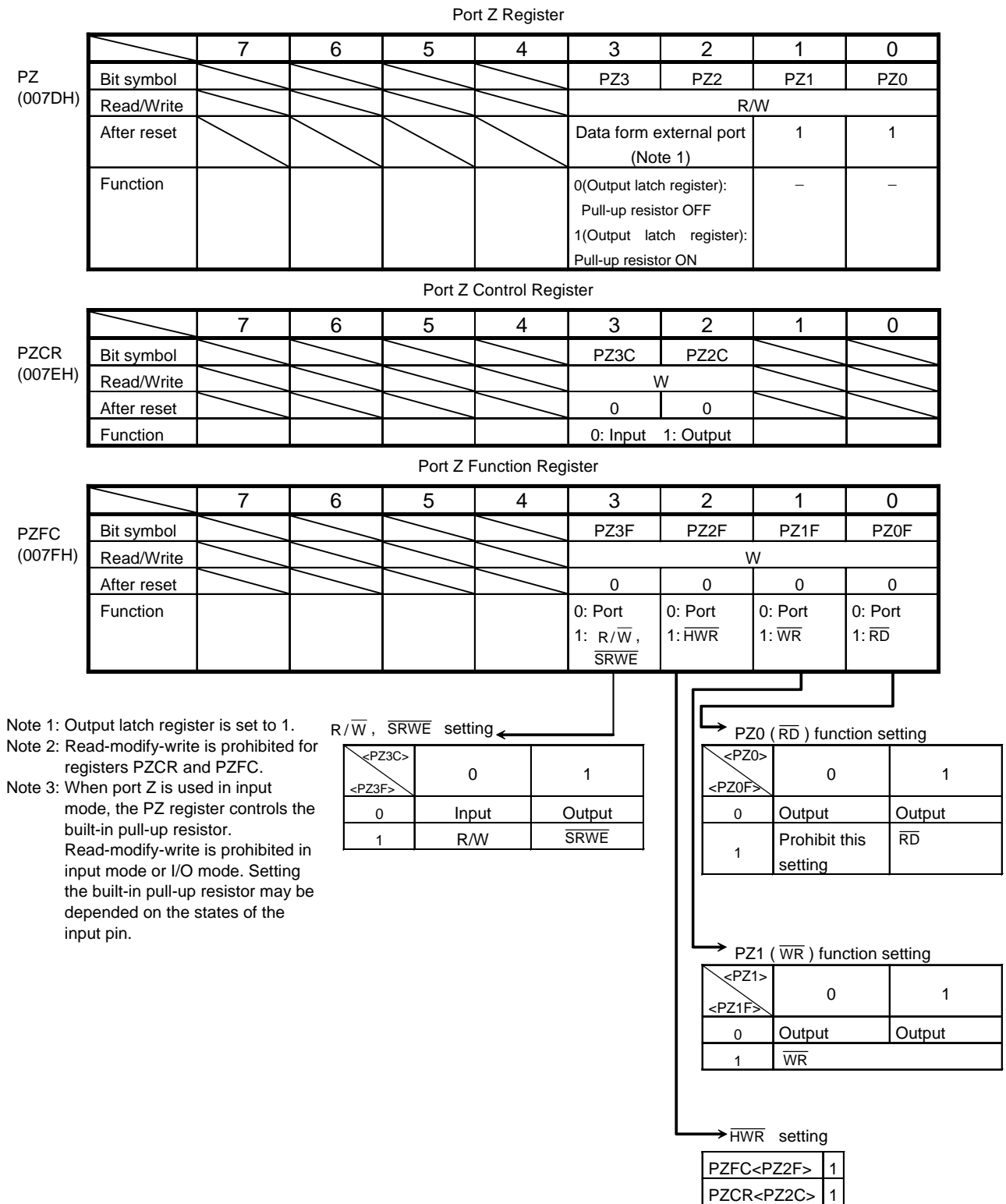
Figure 3.5.14 Register for Port Z
