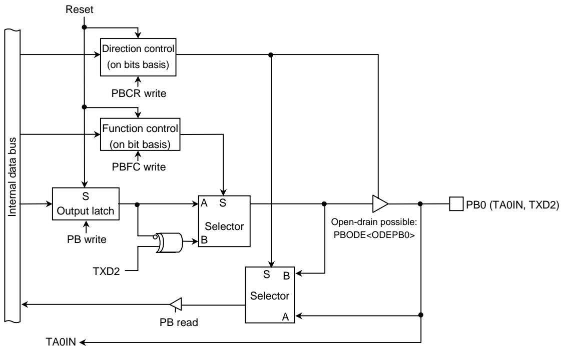
Figure 3.5.31 Port B0
