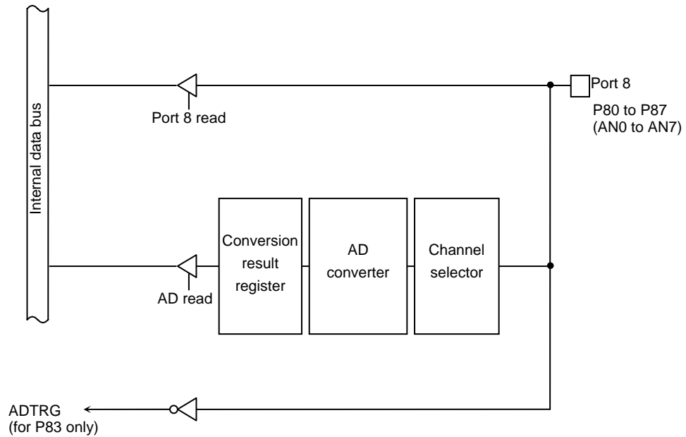
Figure 3.5.25 Port 8
