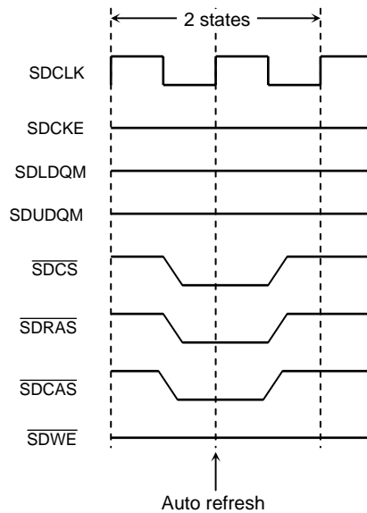
Figure 3.16.8 Refresh Cycle
