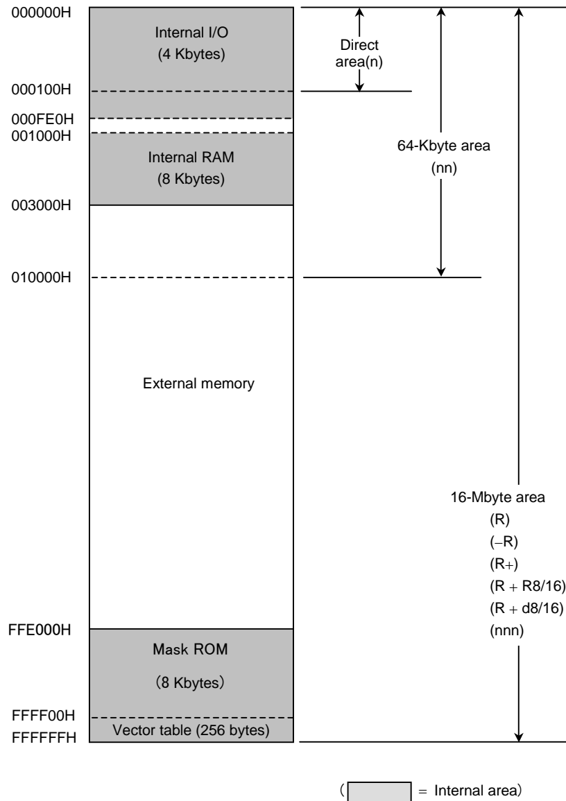
Figure 3.2.1 Memory Map
