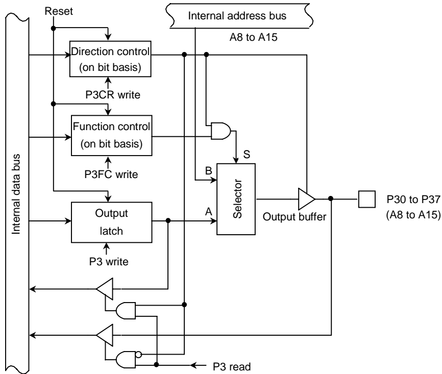
Figure 3.5.7 Port 3
