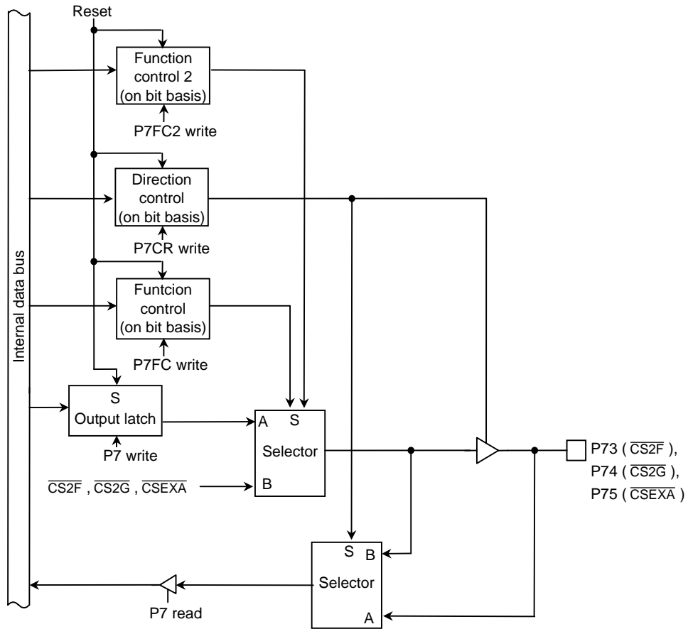
Figure 3.5.22 Port 73, 74, 75
