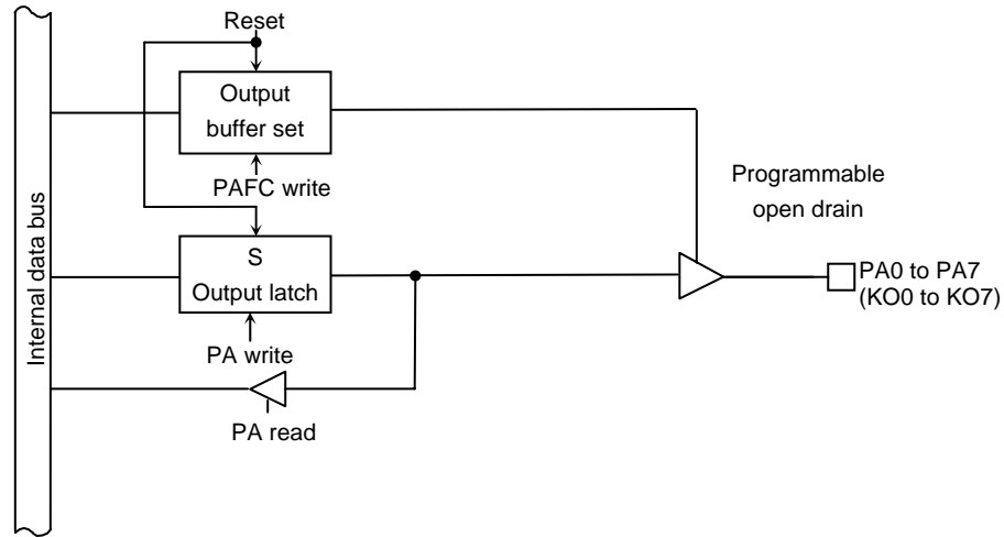
Figure 3.5.29 Port A
