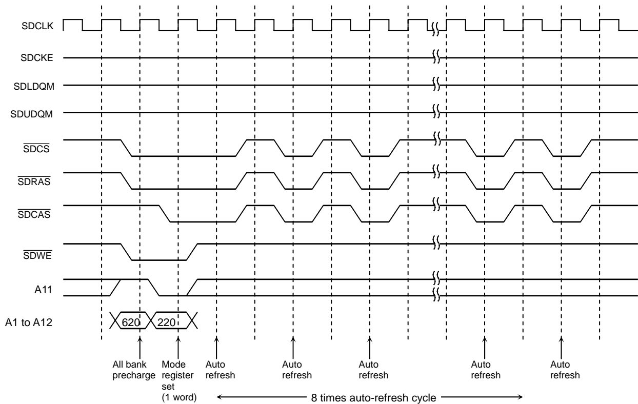
Figure 3.16.10 Initialize Cycle
