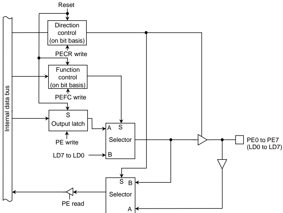
Figure 3.5.43 Port E
