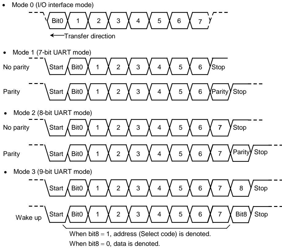
Figure 3.9.1 Data Formats
