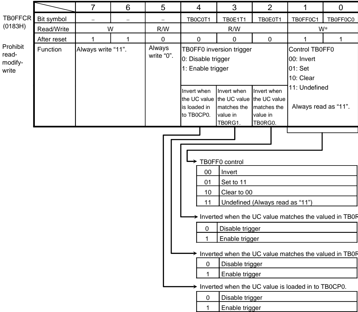
TMRB0 Flip-flop Control Register
