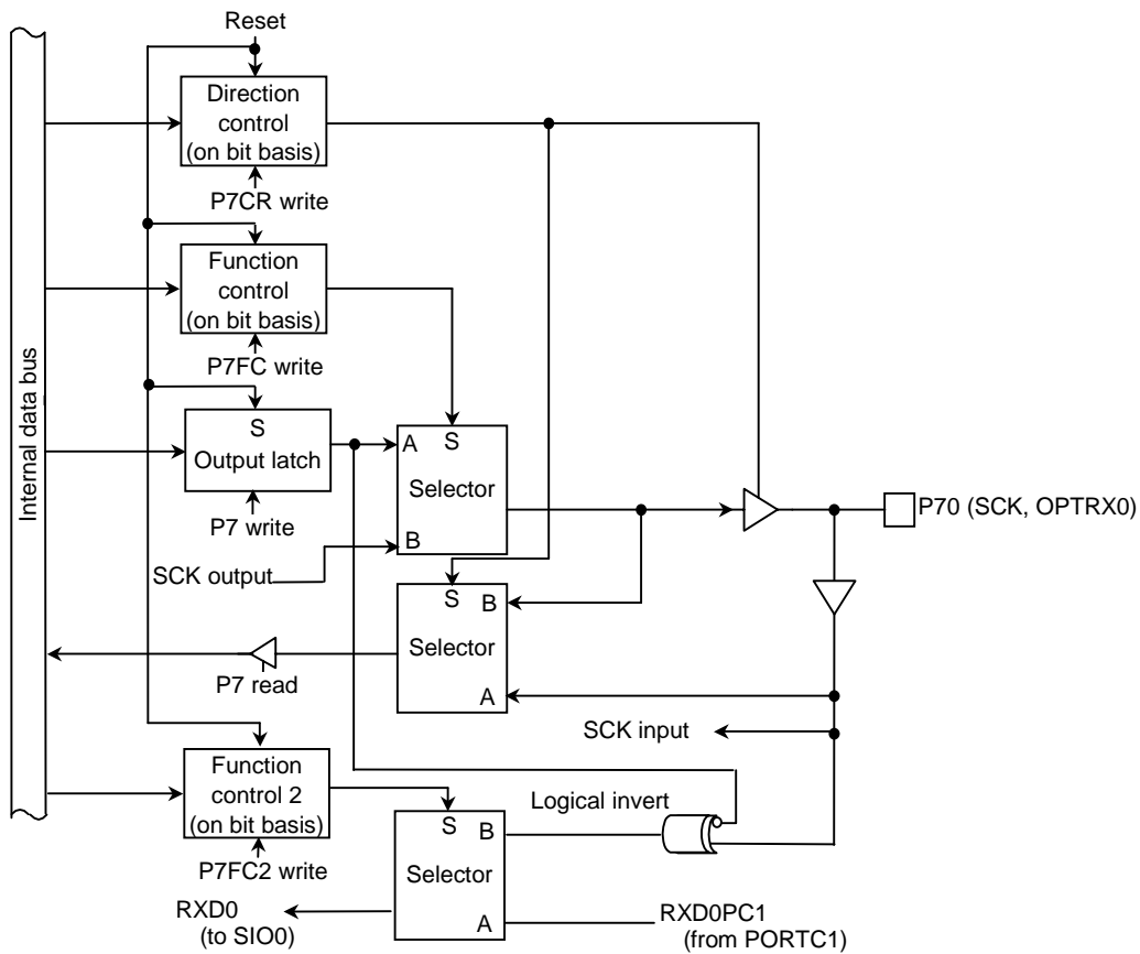
Figure 3.5.19 Port 70
