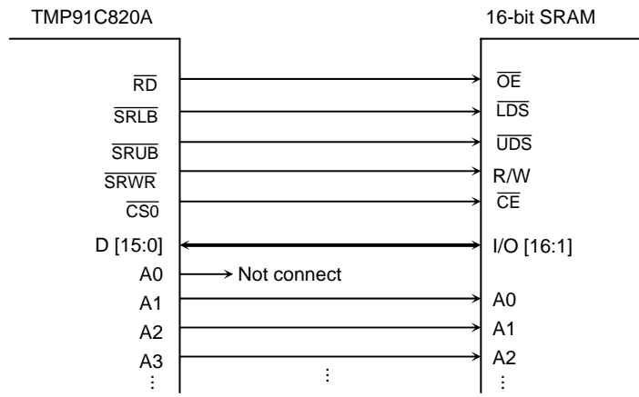
Figure 3.6.7 How to Connect to 16-Bit SRAM for TMP91C820A
