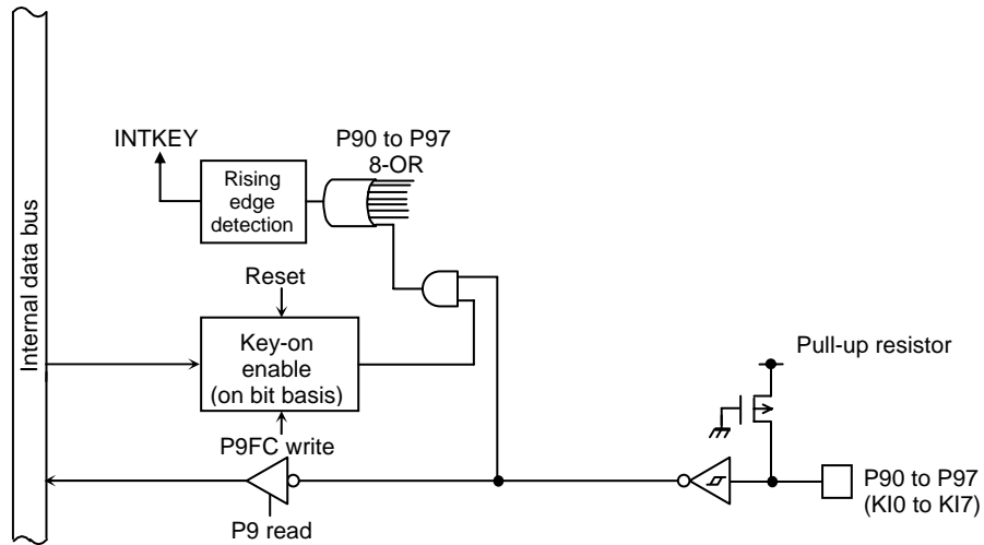
Figure 3.5.27 Port 9
