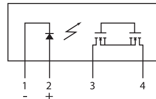
CPC1981Y Pinout
