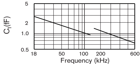
FIGURE 3 CX3H TYPICAL QUALITY FACTOR (Q)
