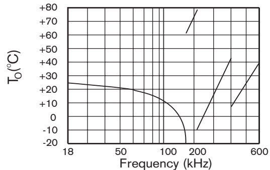
FIGURE 4 CX3H TYPICAL TURNING POINT TEMP. ( T_0 )
