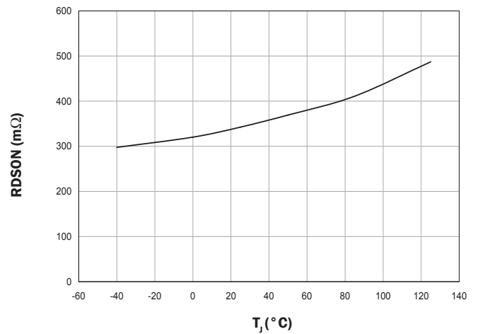
P-Channel R DS(ON) vs. Temperature
