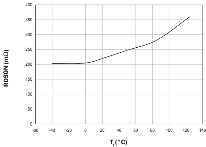
N-Channel R DS(ON) vs. Temperature
