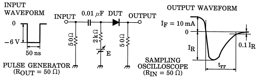
Fig.1 Reverse Recovery Time ( t_{rr} ) Test Circuit
