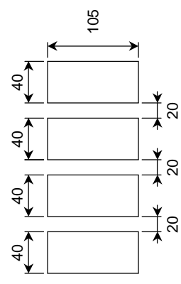
• Long-side power supply PAD (V_GGL/R)
