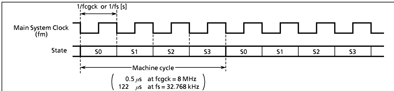
Figure 1-17. Machine Cycle
