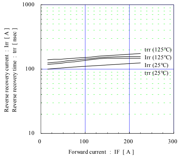
Reverse recovery characteristics (typ.) V_{cc}=600\text{V} , V_{GE}=-15\text{V} , R_g=22\ \text{ohm}
