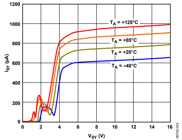
Figure 34. Supply Current vs. Supply Voltage AD8669
