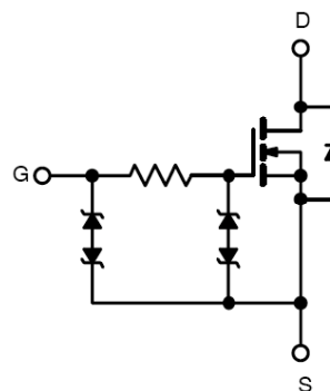
N-Channel MOSFET
