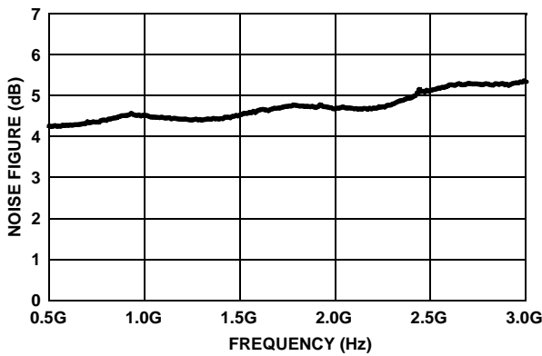
FIGURE 9. NOISE FIGURE vs FREQUENCY
