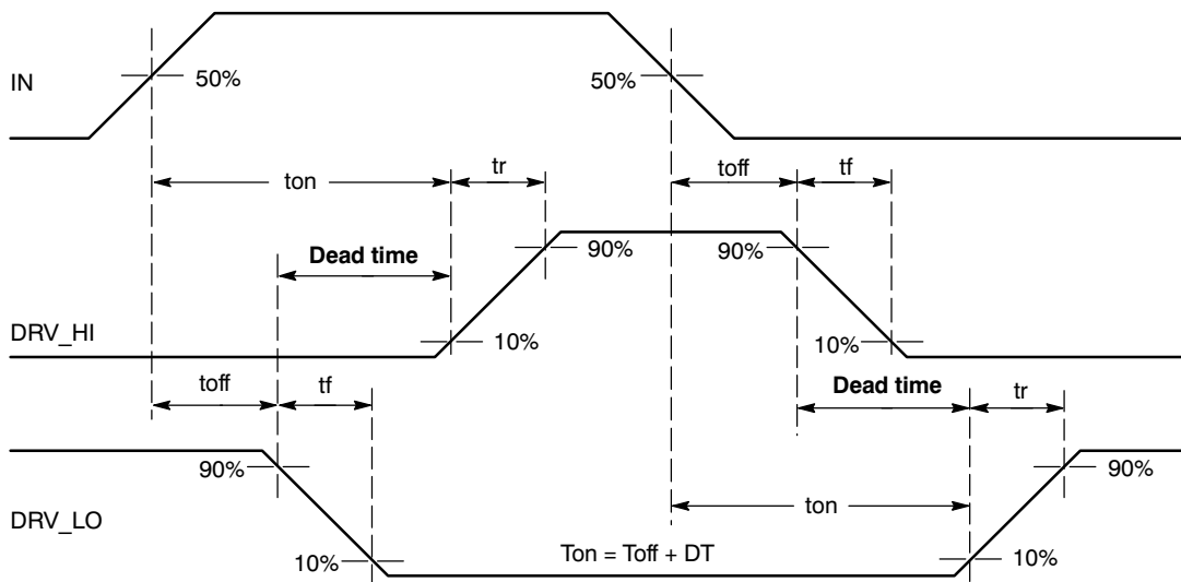
Figure 5. Timing Definitions
