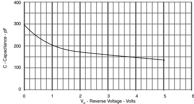
FIGURE 5 TYPICAL REVERSE VOLTAGE VS CAPACITANCE FOR PSD05
