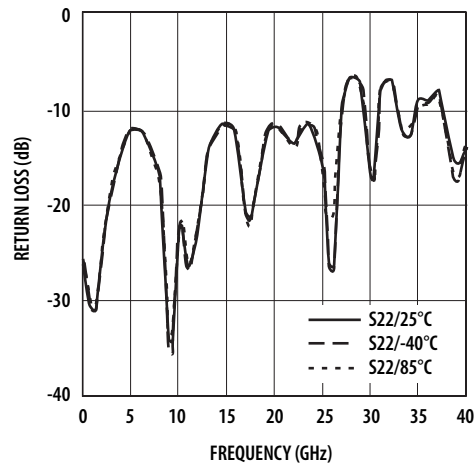
Figure 14. Output Return Loss and Temperature.
