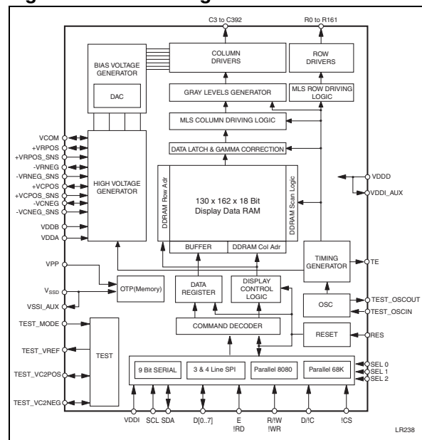
Figure 1. Block diagram
