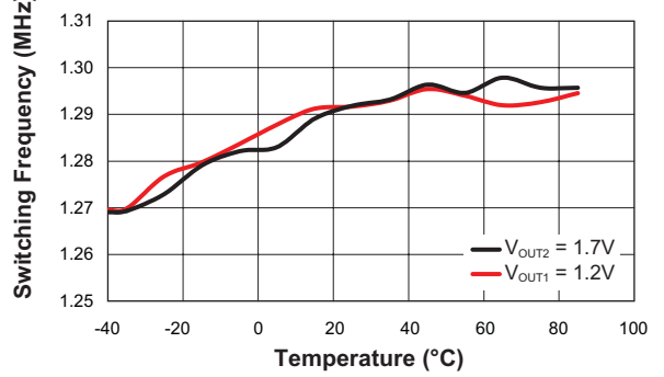
Step-Down Converter Switching Frequency vs. Temperature ( V_{IN} = 3.3V ; I_{OUT1} = 1.2A ; I_{OUT2} = 0.6A )
