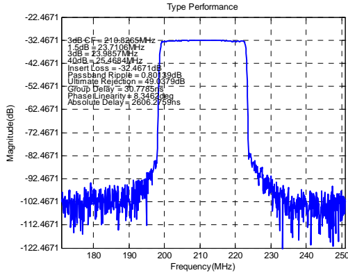
Frequency Response
