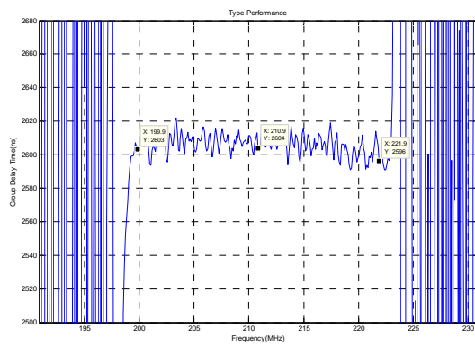
Group Delay Variation (f0±11MHz)
