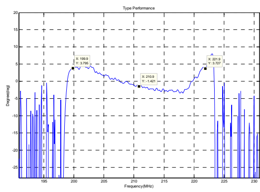
Phase Linearity (f0±11MHz)
