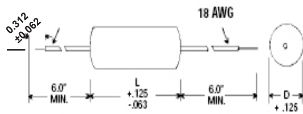
FLEXIBLE LEADS #18 AWG (.040 DIA.)
