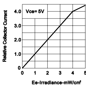
FIG.4 RELATIVE COLLECTOR CURRENT VS IRRADIANCE
