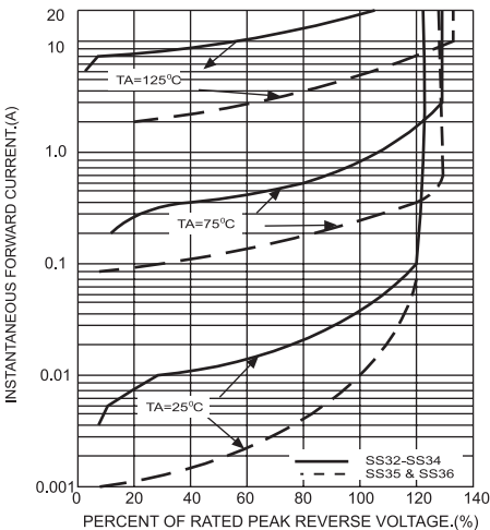
FIG.4-TYPICAL REVERSE CHARACTERISTICS
