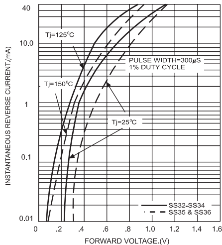
FIG.3-TYPICAL FORWARD CHARACTERISTICS
