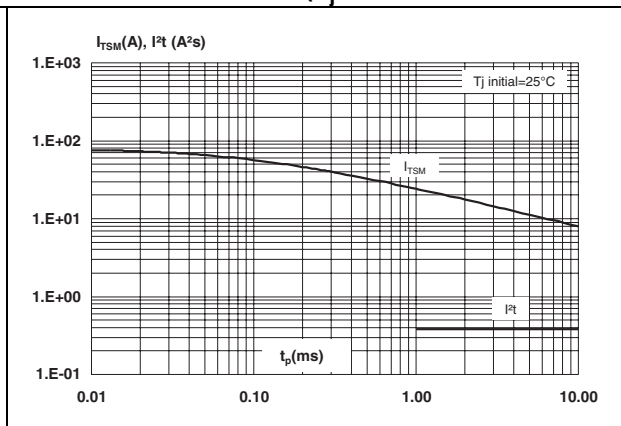
Figure 6. Non repetitive surge peak on-state current for a sinusoidal pulse with width t_p < 10 ms, and corresponding value of I^2t ( T_j initial = 25 ^\circ\text{C} )
