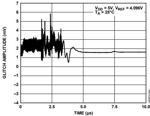
Figure 29. DAC-to-DAC Crosstalk
