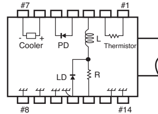
PIN CONNECTIONS
