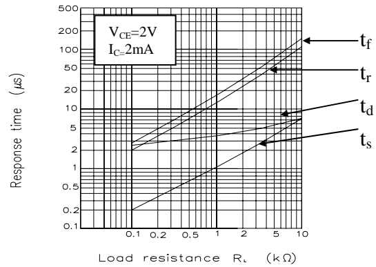
Fig.10 Response Time vs. Load Resistance
