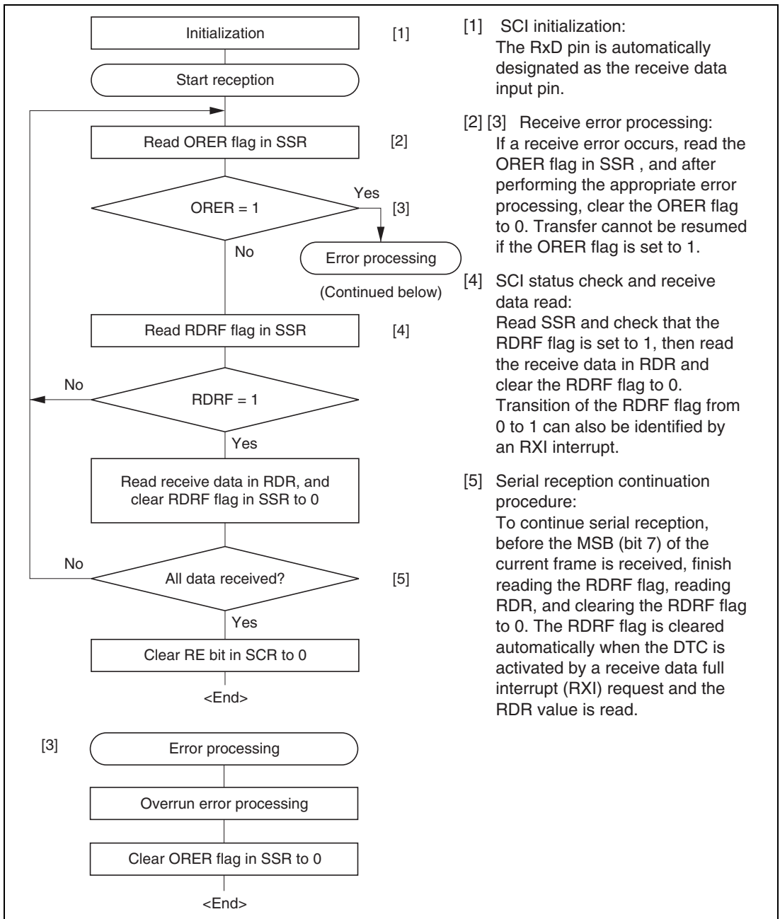
Figure 12.18 Sample Serial Reception Flowchart
