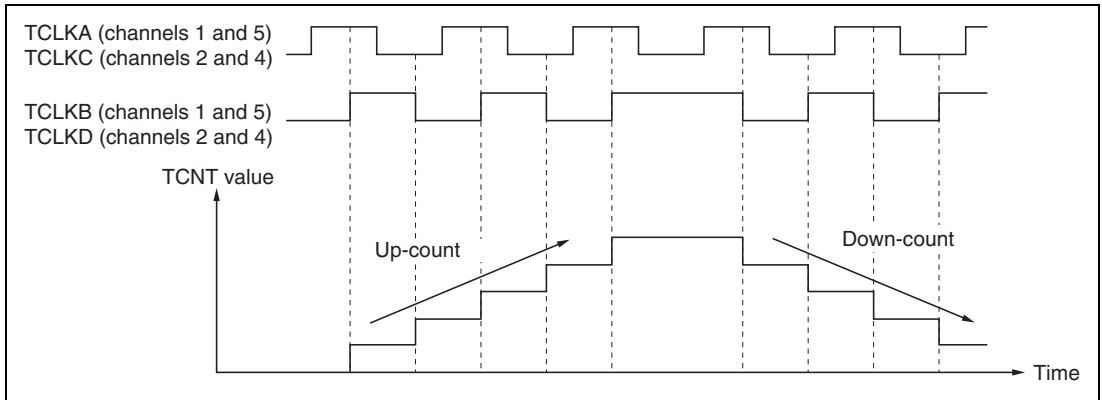
Figure 9.32 Example of Phase Counting Mode 4 Operation
