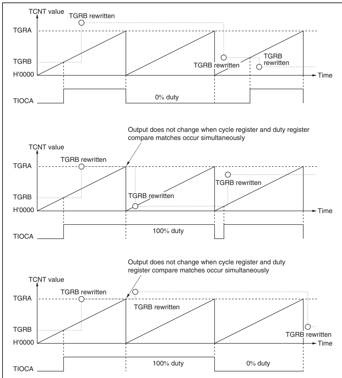
Figure 9.27 Example of PWM Mode Operation (3)
