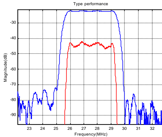
SP27.5-3.4 SAW Filter Typical Performance
