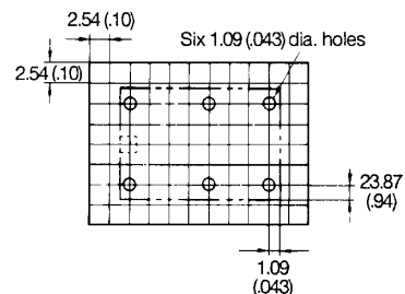
Mounting holes
