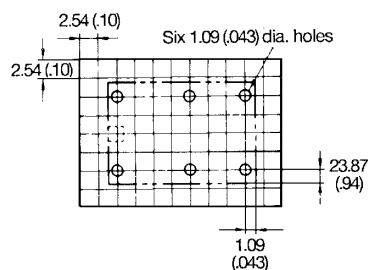
Mounting holes
