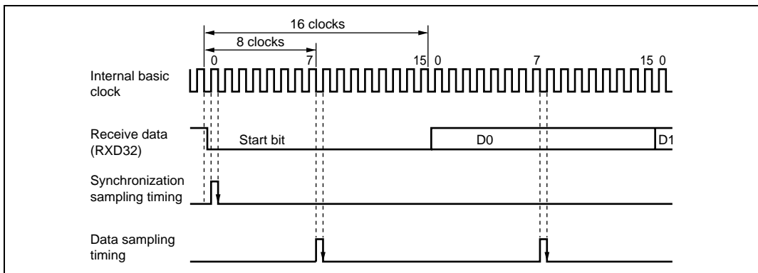
Figure 10.20 Receive Data Sampling Timing in Asynchronous Mode
