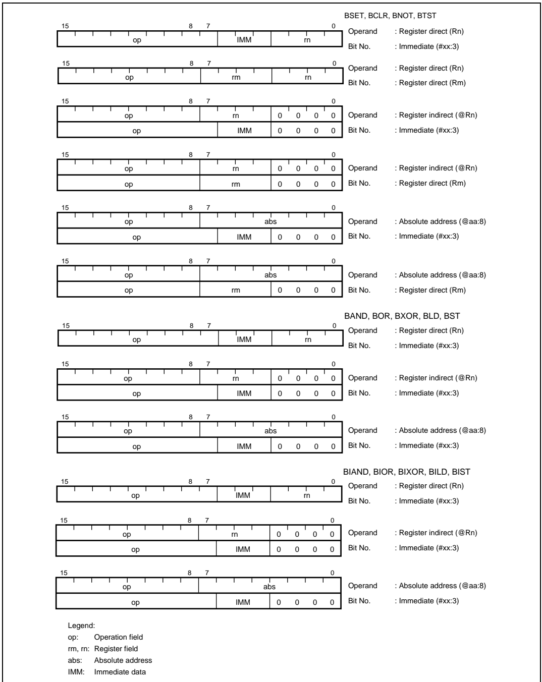
Figure 2.8 Instruction Formats of Bit Manipulation Instructions
