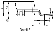
Figure E.2 Package Dimensions (FP-64E)
