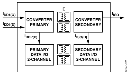
Figure 25. Power Consumption Within the ADuM520x
