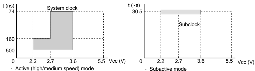
(4) Power supply voltage and instruction executing range (F-ZTAT-version regular specifications/Masked ROM version)
