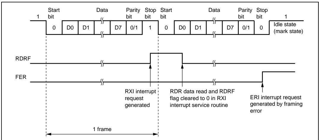
Figure 15.11 Example of SCI Operation in Reception (Example with 8-Bit Data, Parity, One Stop Bit)
