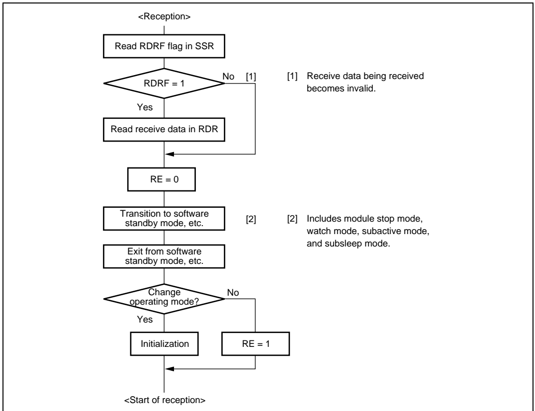
Figure 15.42 Sample Flowchart for Mode Transition during Reception
