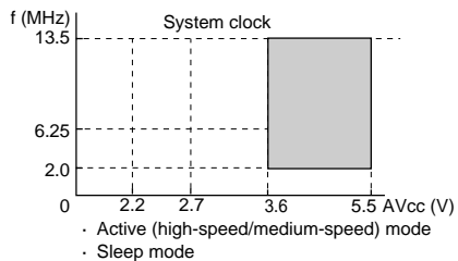
Figure 27.3 Power Supply Voltage and Operating Ranges (H8S/2238B and H8S/2236B)
