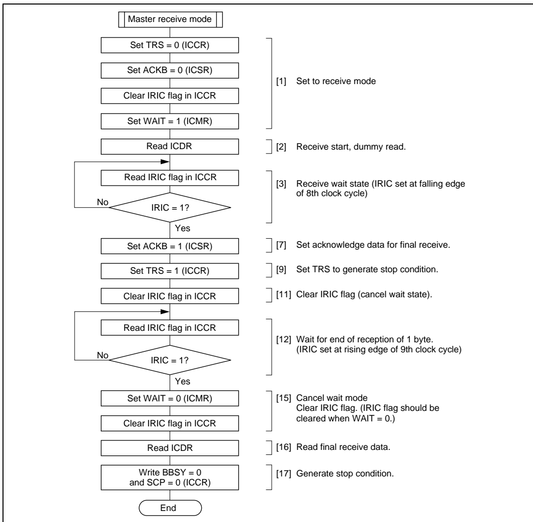
Figure 16.11 Flowchart for Master Receive Mode (Receiving 1 Byte) (WAIT = 1) (Example)
