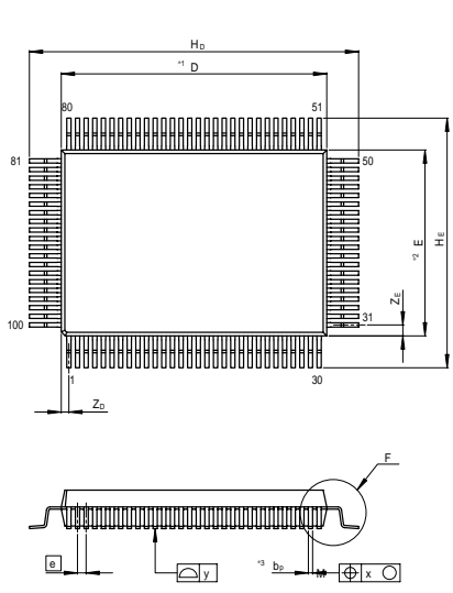
Figure C.3 FP-100A Package Dimensions
