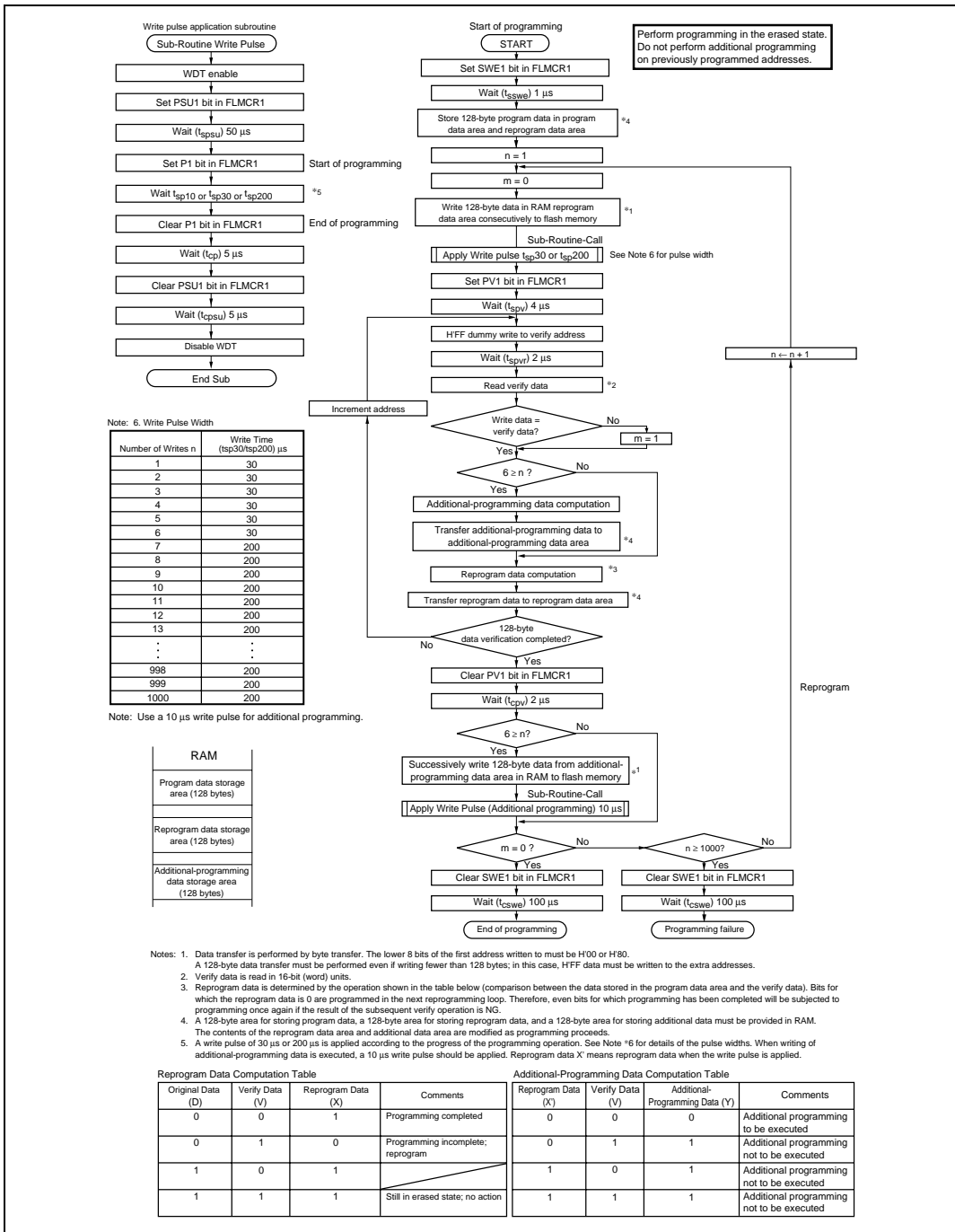
Figure 20.11 Program/Program-Verify Flowchart
