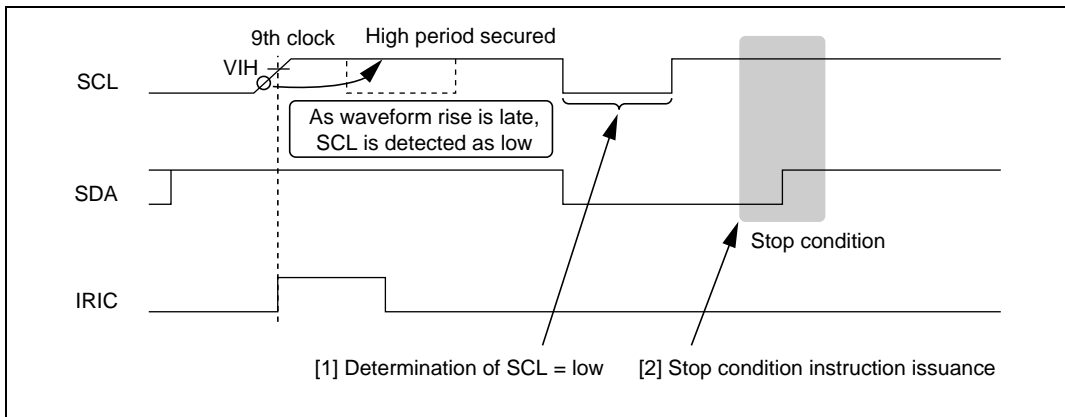
Figure 16.23 Timing of Stop Condition Issuance
