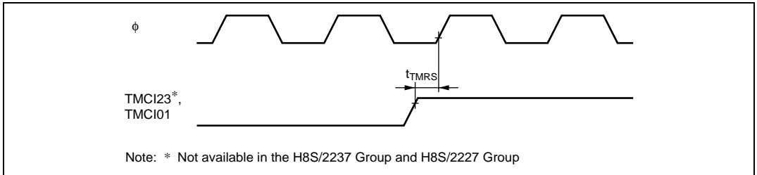
Figure 27.29 8-Bit Timer Reset Input Timing
