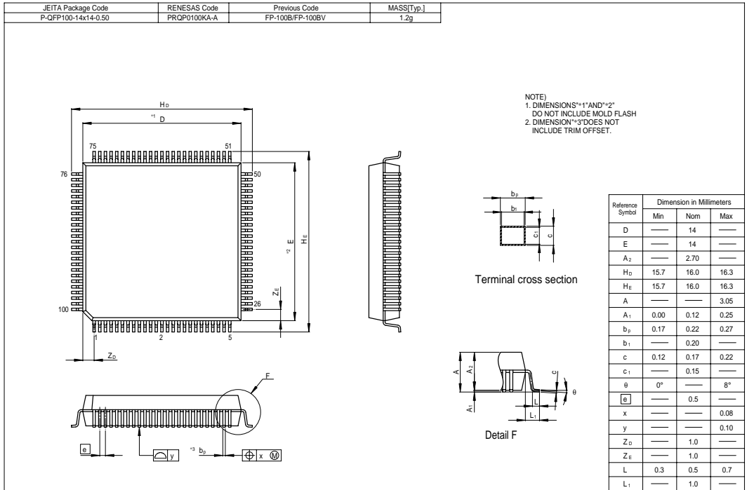
Figure C.4 FP-100B Package Dimensions
