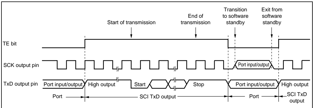
Figure 15.40 Asynchronous Transmission Using Internal Clock
