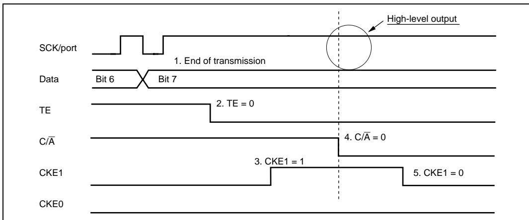
Figure 15.44 Operation when Switching from SCK Pin Function to Port Pin Function (Example of Preventing Low-Level Output)
