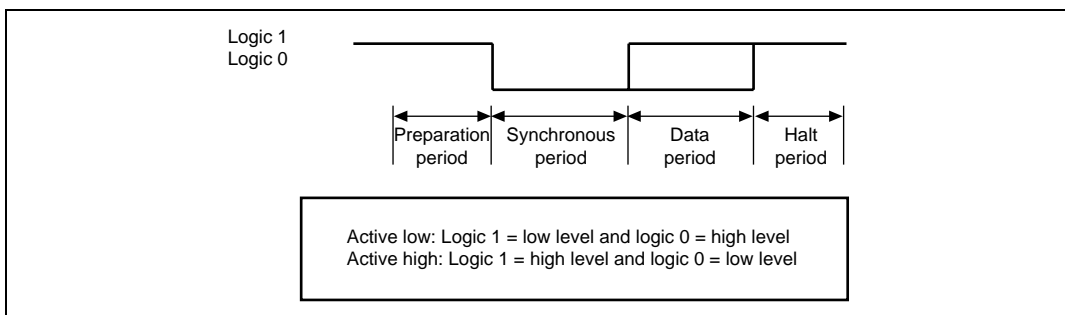
Figure 14.5 IEBus Bit Format (Conceptual Diagram)
