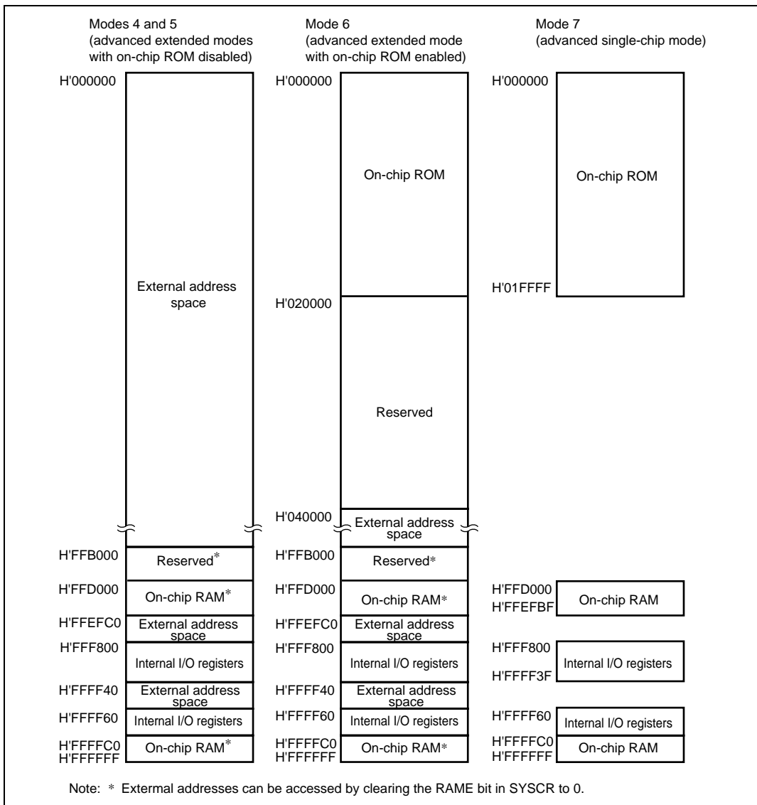
Figure 3.2 H8S/2256 Memory Map in Each Operating Mode
