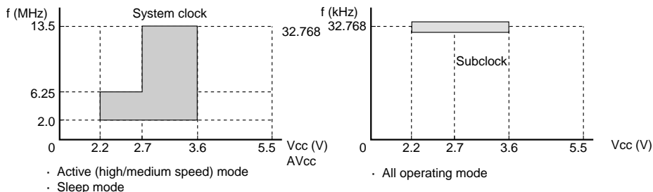
(3) Power supply voltage and instruction executing range (F-ZTAT-version wide-range specifications)
