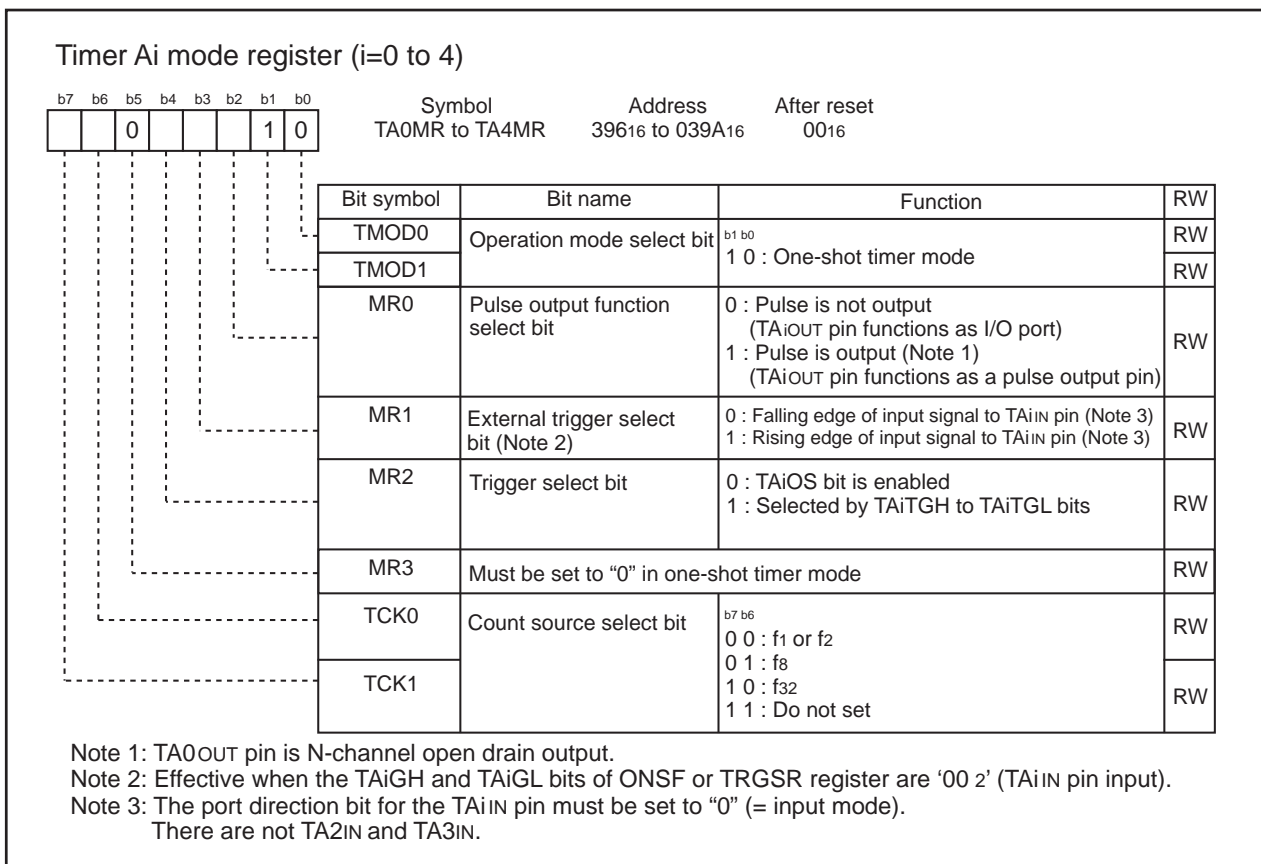
Figure 1.12.10. TA i MR Register in One-shot Timer Mode
