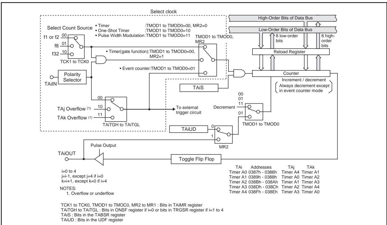
Figure 1.12.2. Timer A Block Diagram
