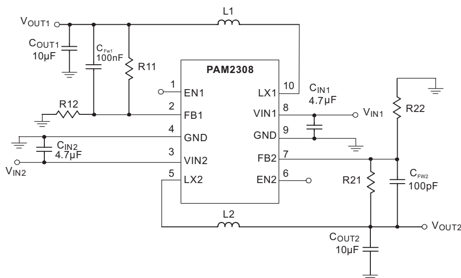
V_{OUTx} = V_{REF} \left( 1 + \frac{R_{x1}}{R_{x2}} \right) Figure 1. Adjustable Voltage Regulator
