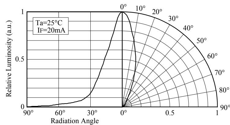
■ Directivity (NSPB310A)
