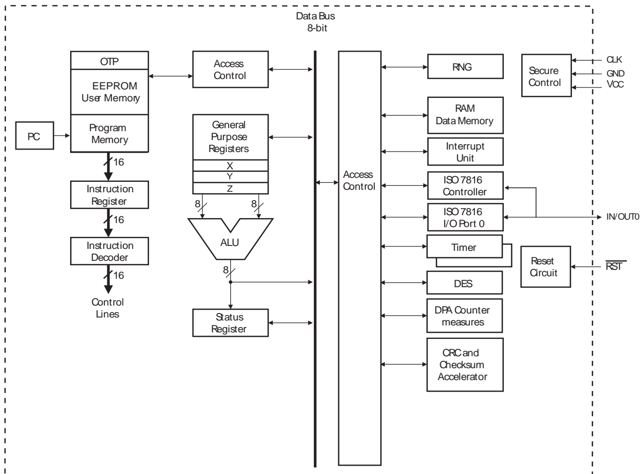
Figure 1. AT90SC9608RT secureAVR RISC Architecture
