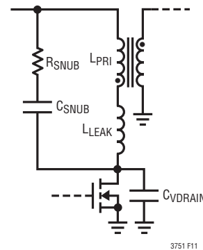
Figure 11. RC Snubber Circuit
