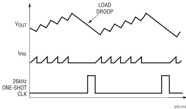
Figure 13. Voltage Ripple Stability Constraint
