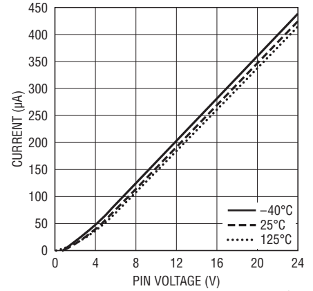
CHARGE Pin Current vs Pin Voltage
