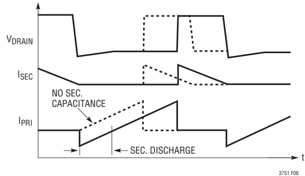
Figure 8. Effect of Secondary Winding Capacitance
