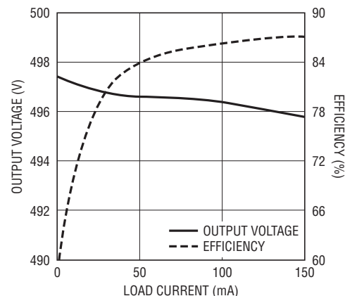
Regulation Mode Load Regulation and Efficiency vs Load Current
