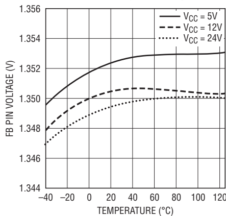
FB Pin Overvoltage Mode Threshold Voltage vs Temperature
