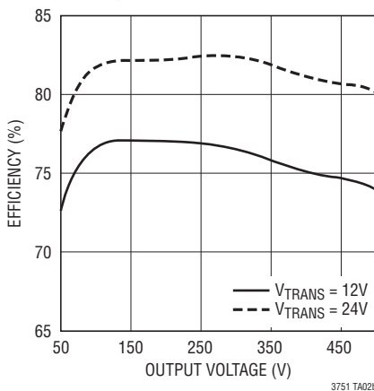
Charging Efficiency vs Output Voltage
