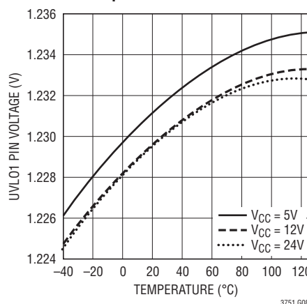
UVLO1 Trip Voltage vs Temperature
