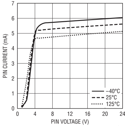
V CC Pin Current vs Pin Voltage
