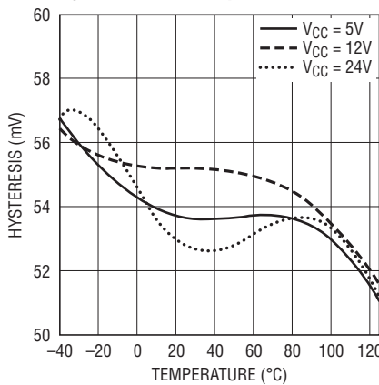
FB Pin Regulation Mode Hysteresis vs Temperature
