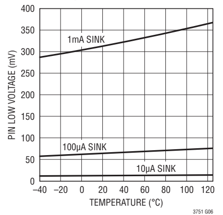
DONE, FAULT Pin Voltage Low vs Temperature
