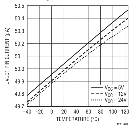
UVLO1 Trip Current vs Temperature
