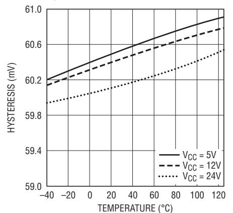
FB Pin Overvoltage Mode Hysteresis vs Temperature
