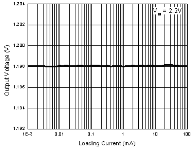
Fig. 8 Output Voltage VS Loading Current (1.2V)
