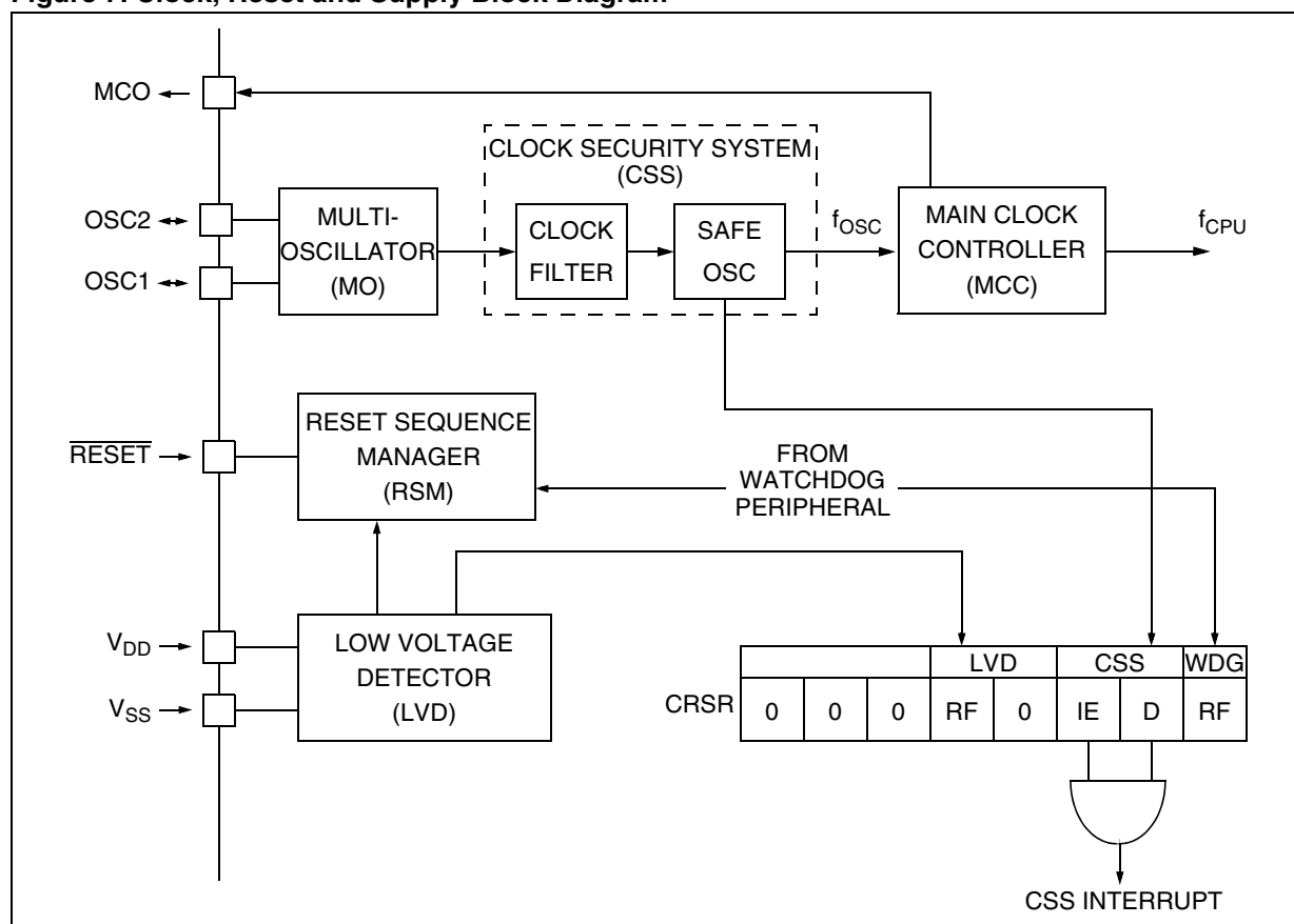
Figure 7. Clock, Reset and Supply Block Diagram
