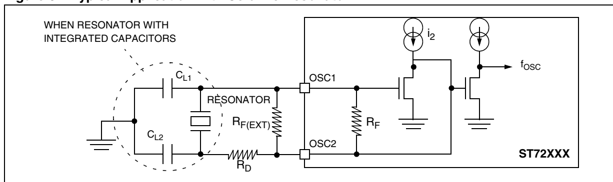
Figure 64. Typical Application with Ceramic Resonator
