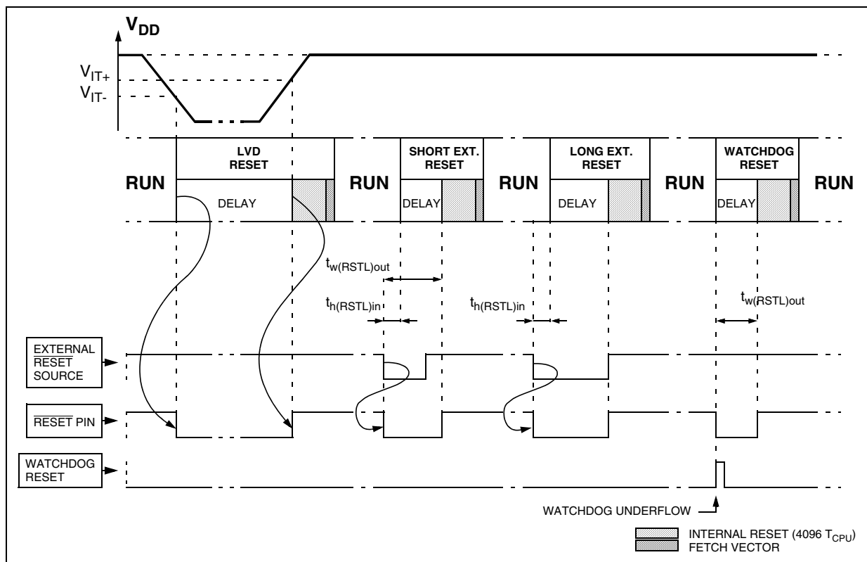
Figure 11. RESET Sequences
