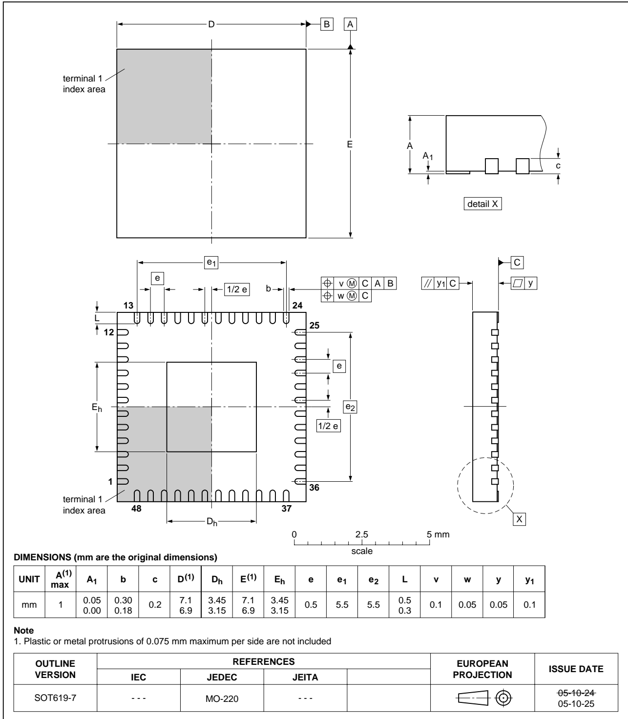
Fig 7. Package outline SOT619-7 (HVQFN48)
