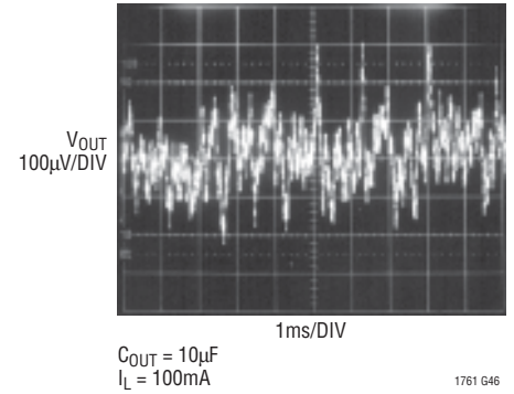
LT1761-5 10Hz to 100kHz Output Noise C_{\text{BYF}} = 100\text{pF}
