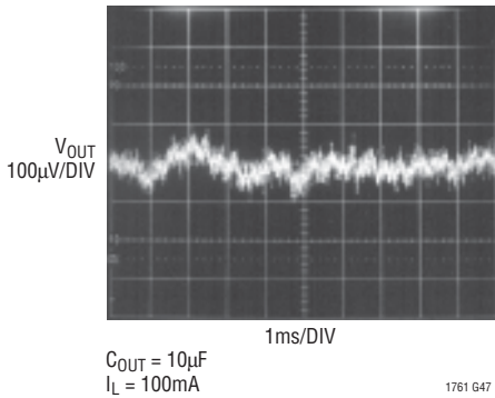
LT1761-5 10Hz to 100kHz Output Noise C_{\text{BYF}} = 1000\text{pF}
