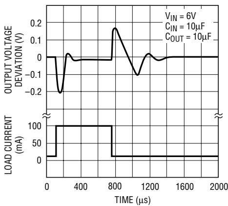
LT1761-5 Transient Response C_{\text{BYF}} = 0
