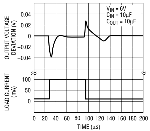
LT1761-5 Transient Response C_{\text{BYF}} = 0.01\mu\text{F}
