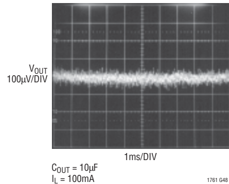
LT1761-5 10Hz to 100kHz Output Noise C_{\text{BYF}} = 0.01\mu\text{F}
