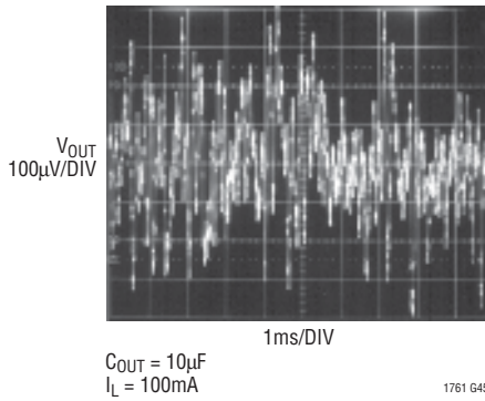
LT1761-5 10Hz to 100kHz Output Noise C_{\text{BYF}} = 0
