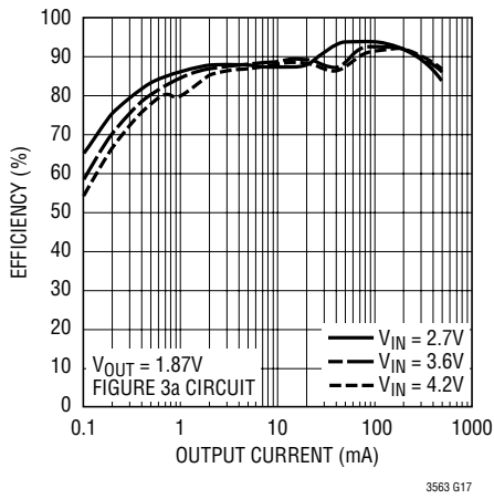
Figure 3c. Efficiency Curve
