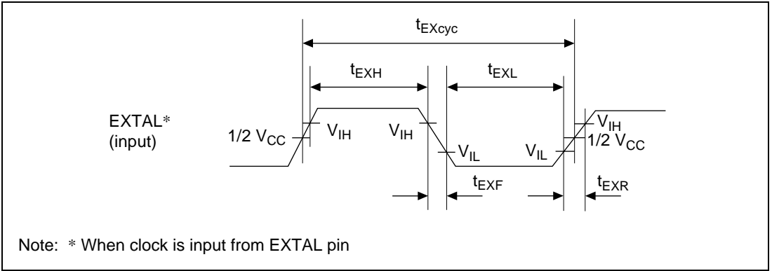
Figure 21.1 EXTAL Clock Input Timing
