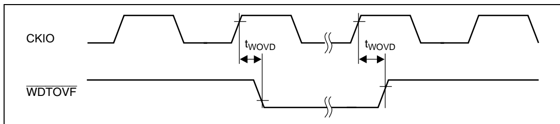
Figure 21.59 Watchdog Timer Output Timing ( t_{Eyc}:t_{Pcyc} = 1:1 )
