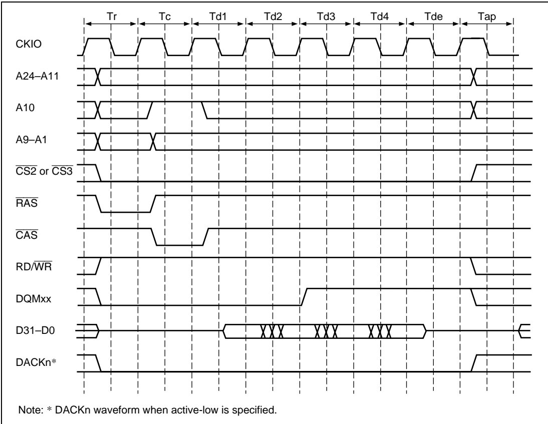
Figure 7.21 (a) Single Read Timing (Auto-Precharge) Except t_{E_{eye}}:t_{P_{eye}} 1:1
