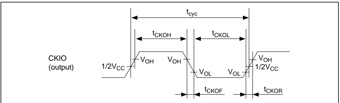
Figure 21.3 CKIO Clock Output Timing
