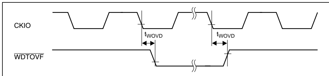
Figure 21.60 Watchdog Timer Output Timing (Except t_{Eyc}:t_{Pcyc} 1:1 )
