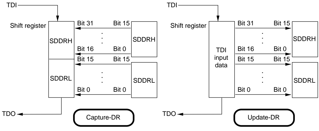
Figure 17.6 Serial Data Input/Output (2)
