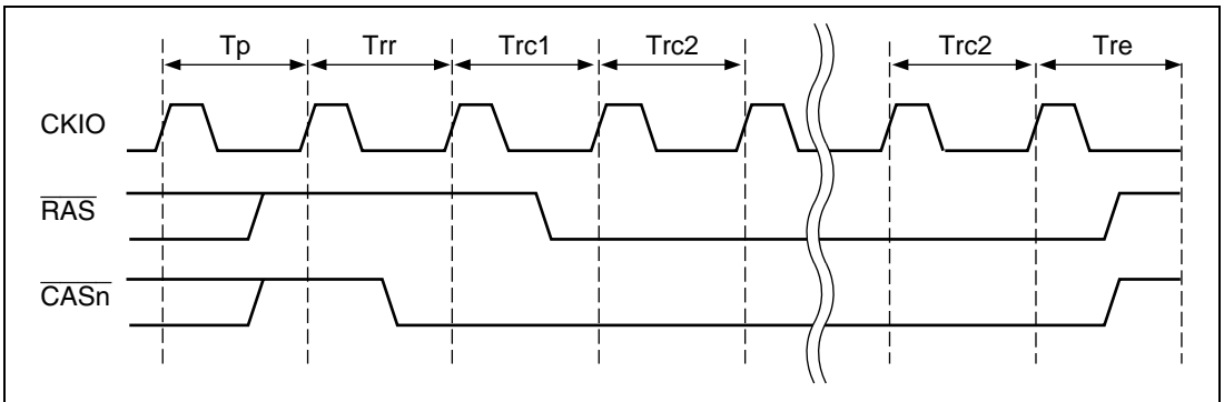
Figure 7.52 DRAM Self-Refresh Cycle Timing
