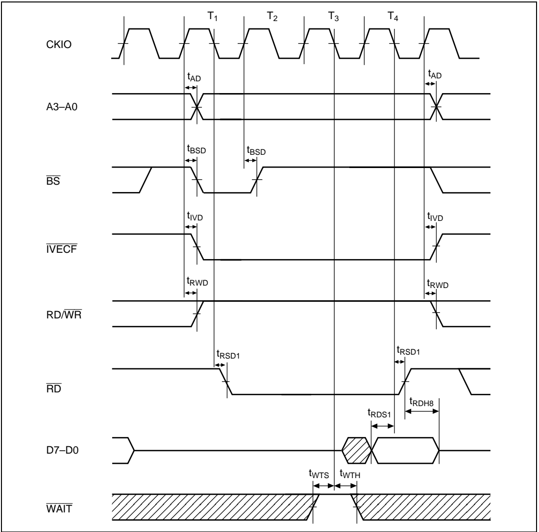
Figure 21.44 Interrupt Vector Fetch Cycle (No Wait, I \phi :E \phi = 1:1)
