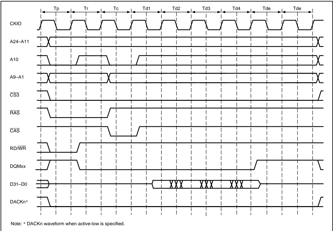
Figure 7.26 (b) Burst Read Timing (Bank Active, Different Row Addresses) Iφ:Eφ = 1:1
