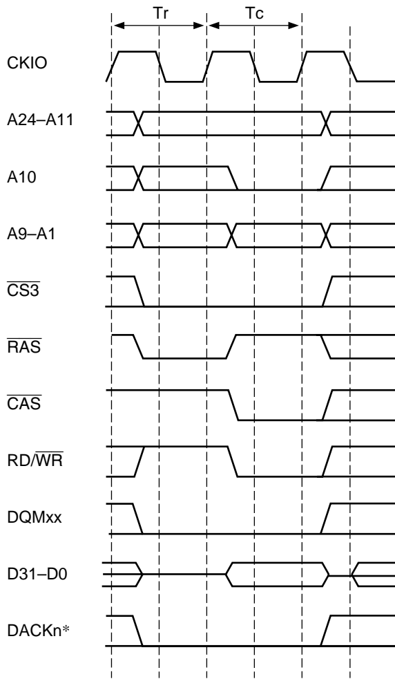
Figure 7.27 Single Write Mode Timing (No Precharge)
