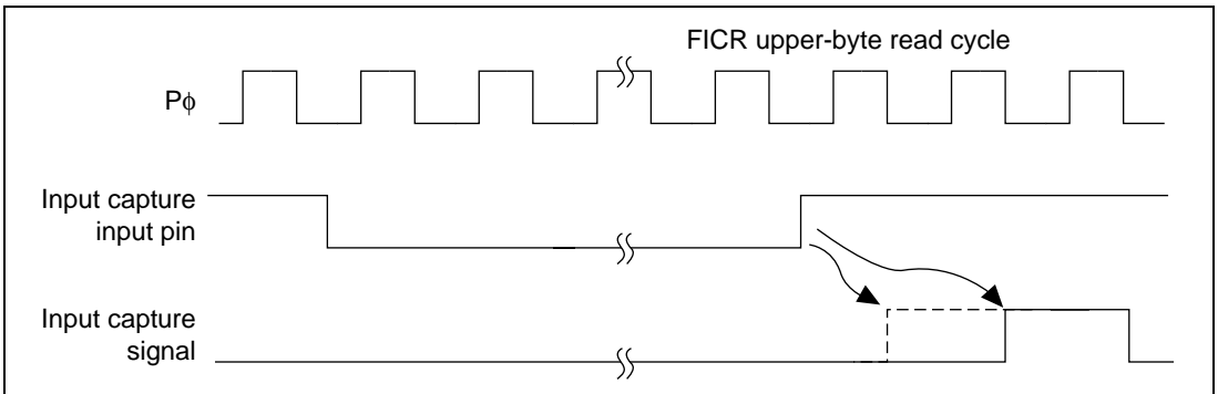
Figure 12.9 Input Capture Signal Timing (Input Capture Input when FICR is Read)
