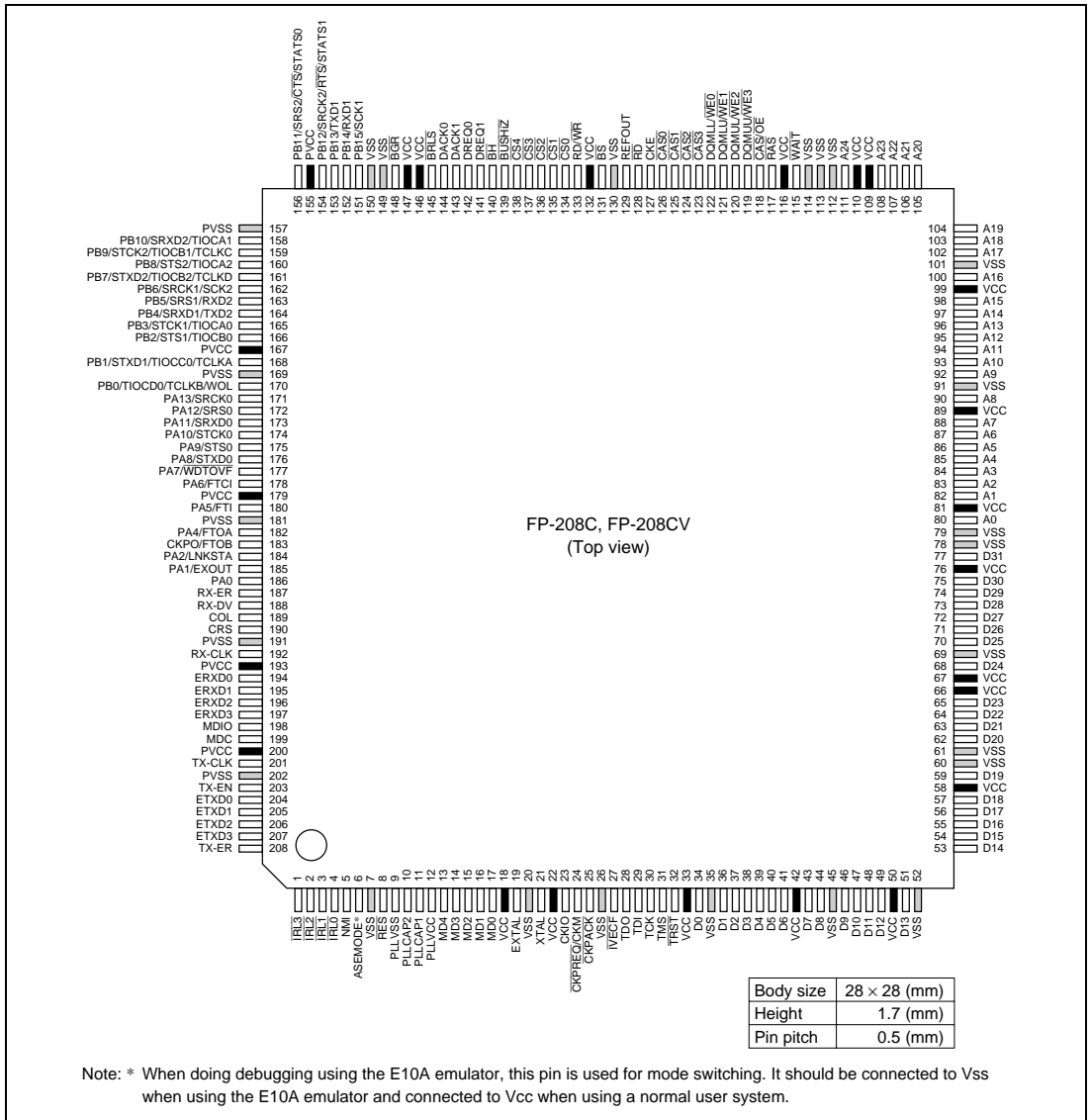
Figure 1.2 HD6417615ARF and HD6417615ARFV Pin Arrangement (FP-208C, FP-208CV)
