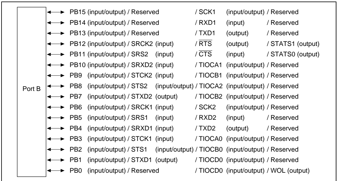
Figure 19.2 Port B
