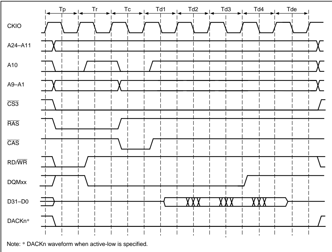
Figure 7.26 (a) Burst Read Timing (Bank Active, Different Row Addresses) Except t_{E_{eye}}:t_{P_{eye}} 1:1
