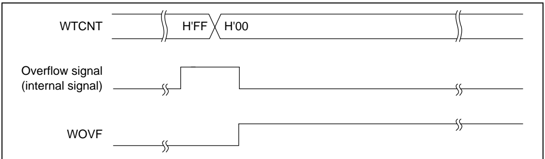
Figure 13.7 Timing of WOVF Setting
