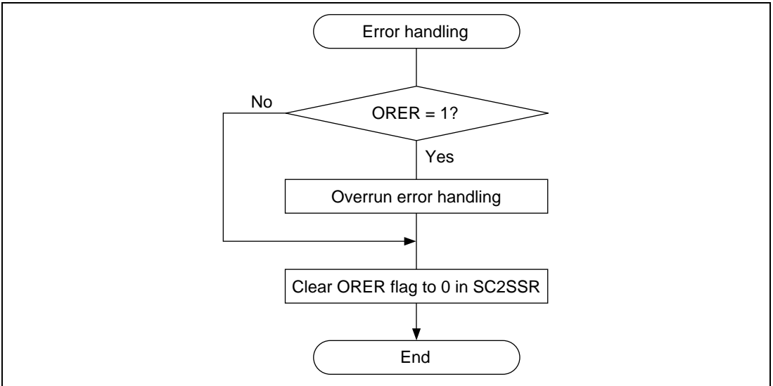
Figure 14.20 Sample Serial Reception Flowchart (2)
