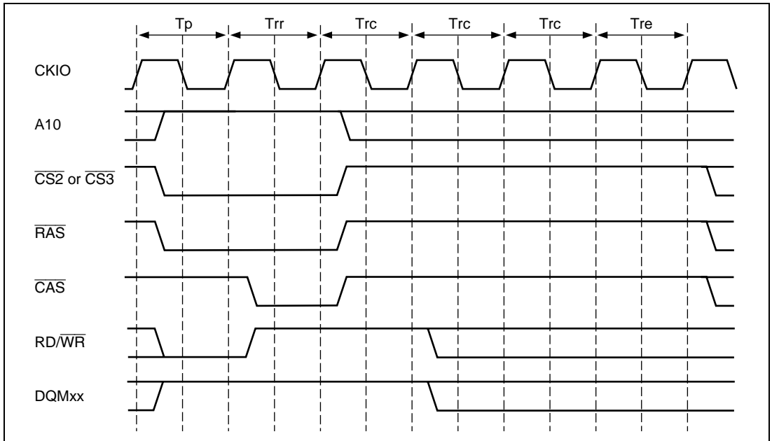
Figure 7.30 Auto-Refresh Timing
