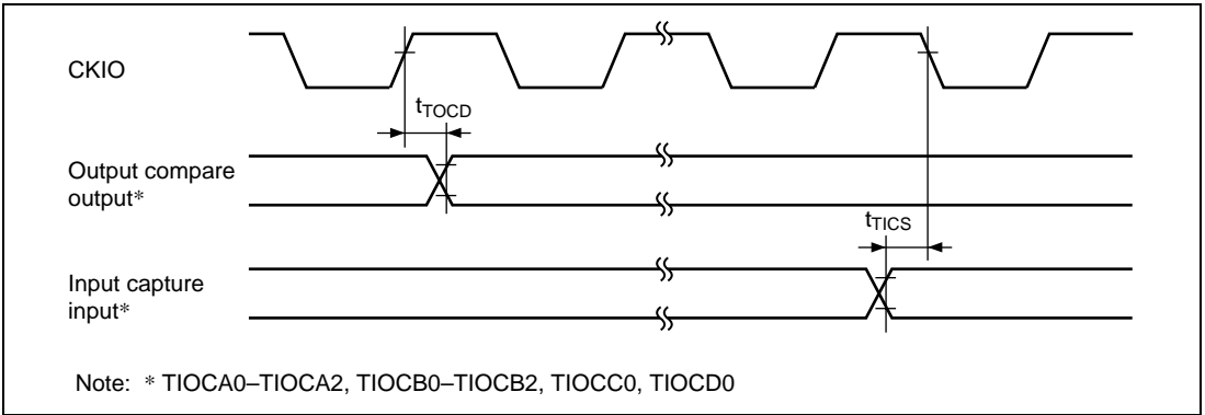
Figure 21.56 TPU Input/Output Timing ( t_{E_{cyc}}:t_{P_{cyc}} = 1:1 )
