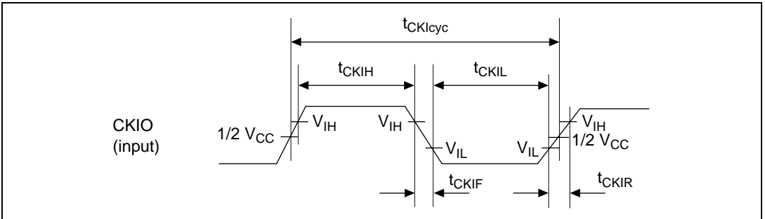
Figure 21.2 CKIO Clock Input Timing
