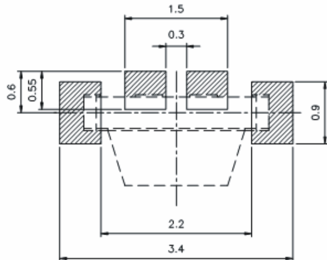
For reflow soldering (propose)
