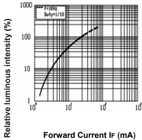
Luminous Intensity vs. Forward Current T_a = 25^\circ
