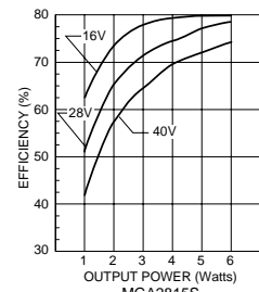
Typical Performance Curves: 25°C Tc, 28 VDC Vin, 100% load, unless otherwise specified.
