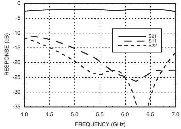
Bypass Mode Broadband Gain & Return Loss [2]
