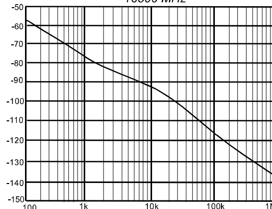
Phase Noise (dBc/Hz) 16500 MHz
