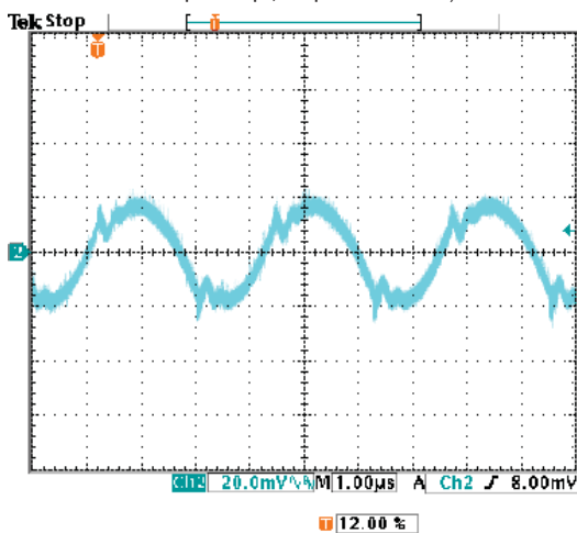
OKX2-T/16-D12 Output Ripple and Noise (Vin=12V, Vout=5V, Iout=16A, Cin=1000µF, Cload=1µF // 10µF, ScopeBW=100MHz)
