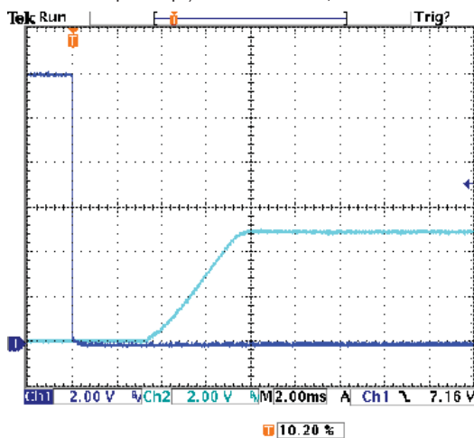
OKX2-T/16-D12-C On/Off Enable Startup Delay (Vin=12V, Vout=5V, Iout=16A, Cin=1000µF, Cload=1µF // 10µF) Trace 1=Enable In, Trace 2=Vout
